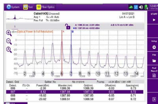
Optical Spectrum Analysis
