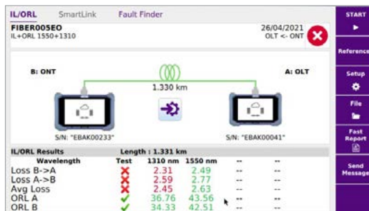
Simplex single fiber test
