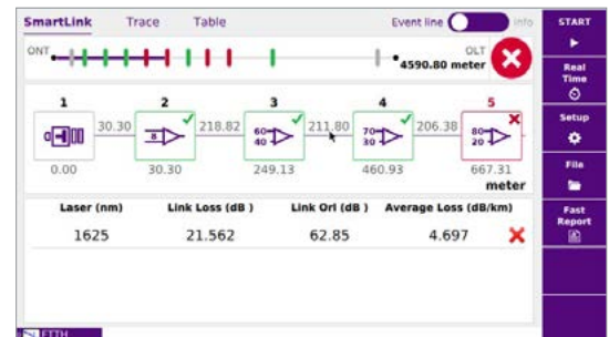
Unbalance/tap splitter network
