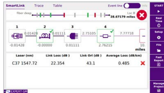
xWDM Link Mapping
