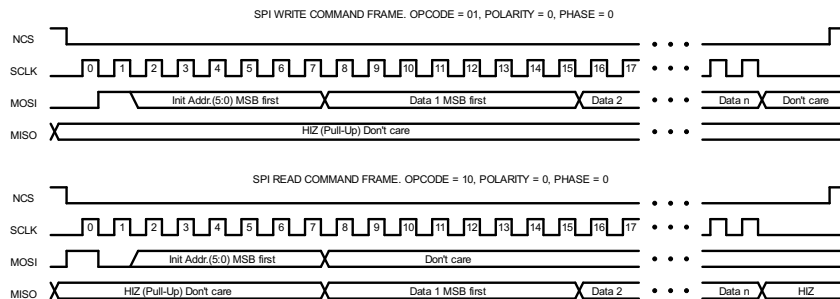
Figure 7: SPI commands
