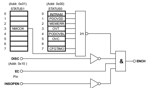
Figure 2: Laser control logic
